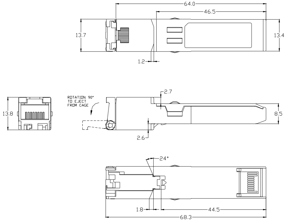
Figure 2. Mechanical Dimensions of Transceiver
